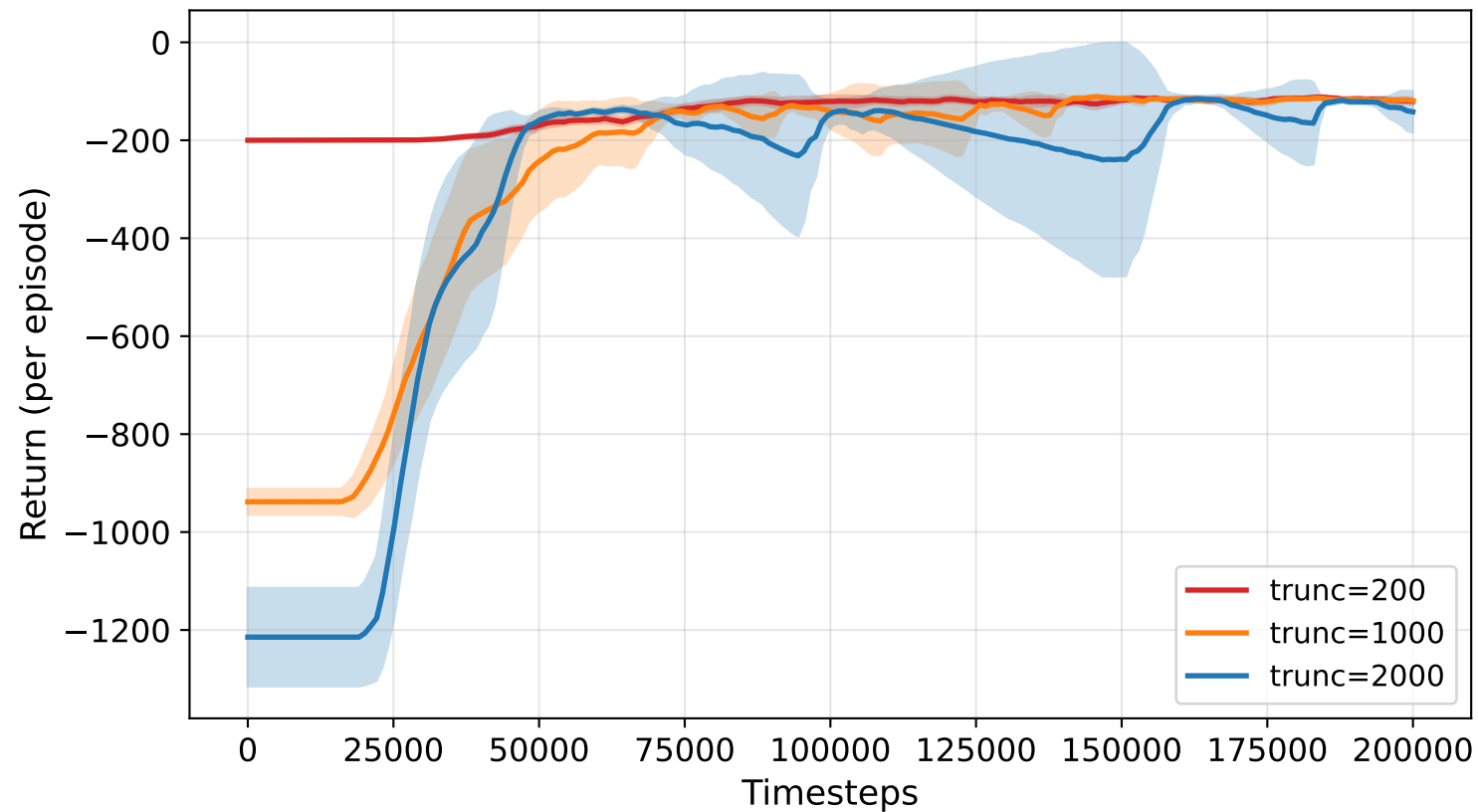
DQN on MountainCar-v0: Effect of Truncation Length (mean \pm 95% CI, 15 seeds)
